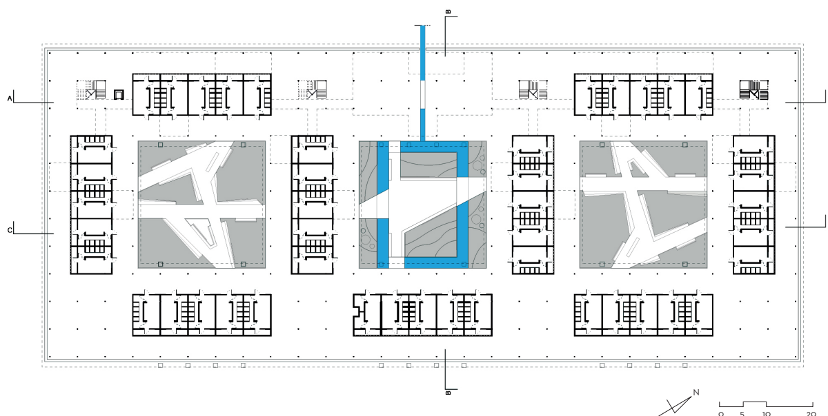
GRUNDRISS | PLAN
