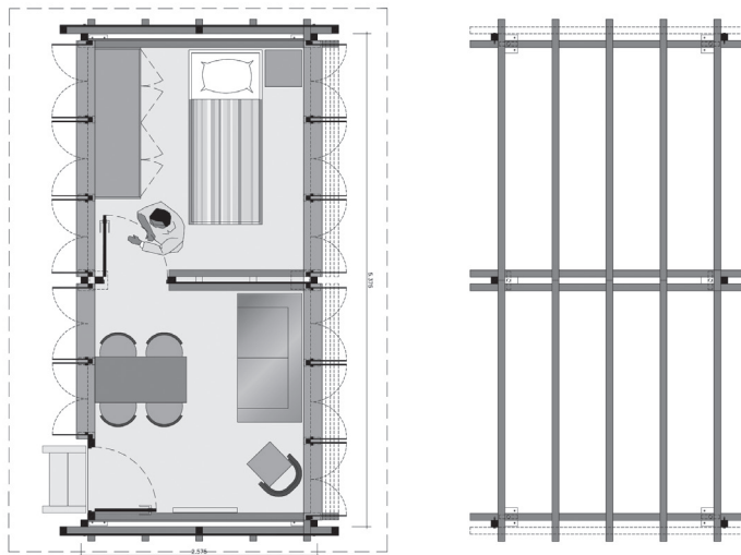
GRUNDRISS | PLAN
